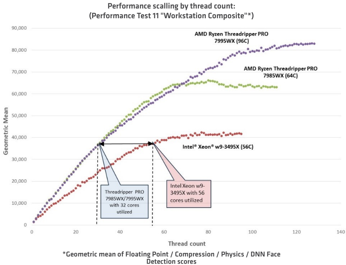
Figure 7: AMD Ryzen Threadripper PRO 7995WX and 7985WX performance scaling by thread count (xi,xiii)
